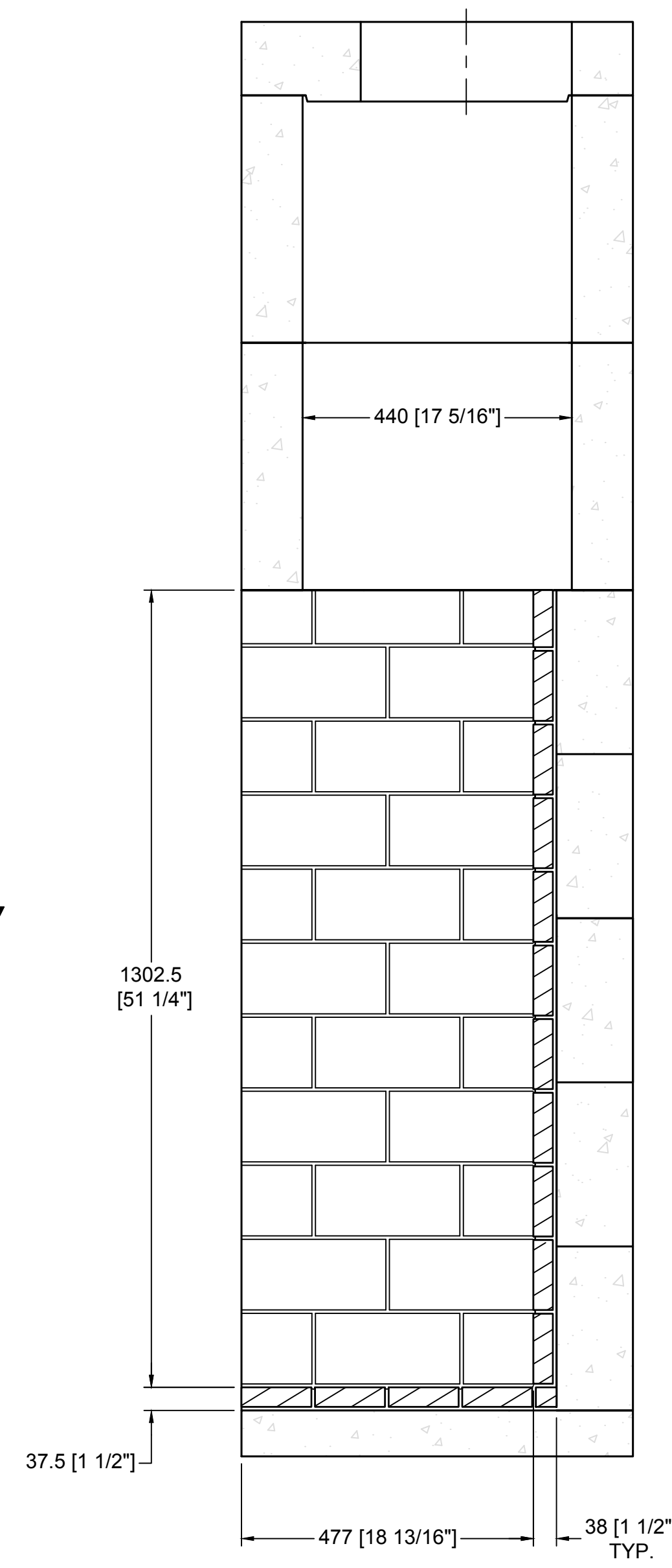
SECTION A-A VERTICAL FIREBRICK DETAIL
