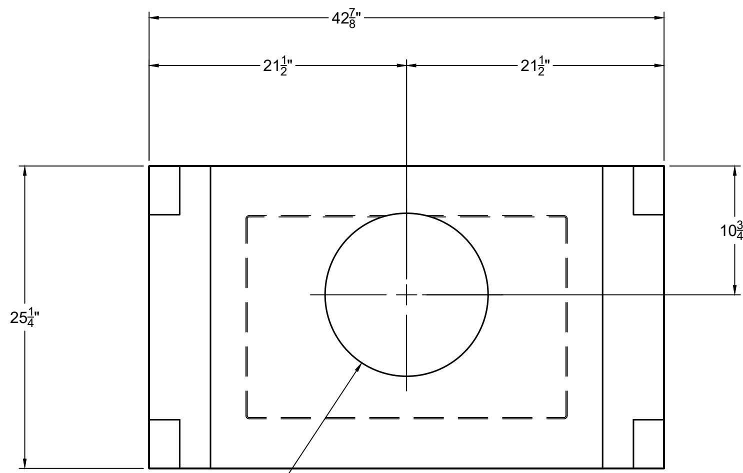
TOP VIEW
