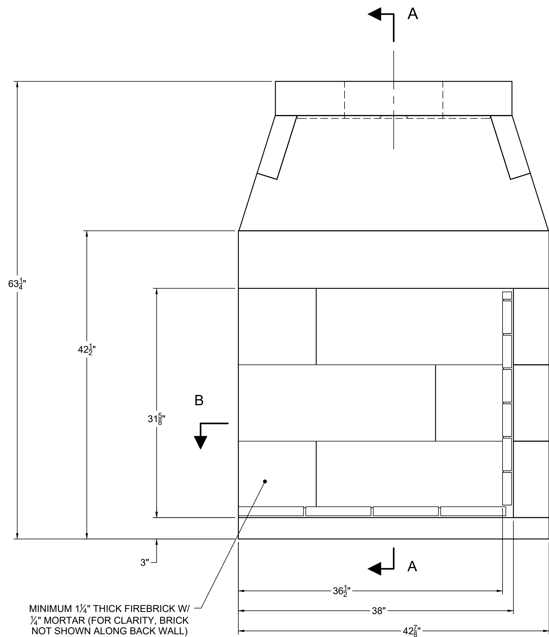
FRONT VIEW
