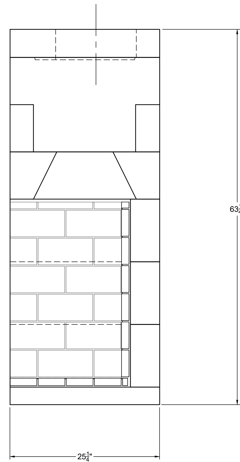
RIGHT-SIDE VIEW
