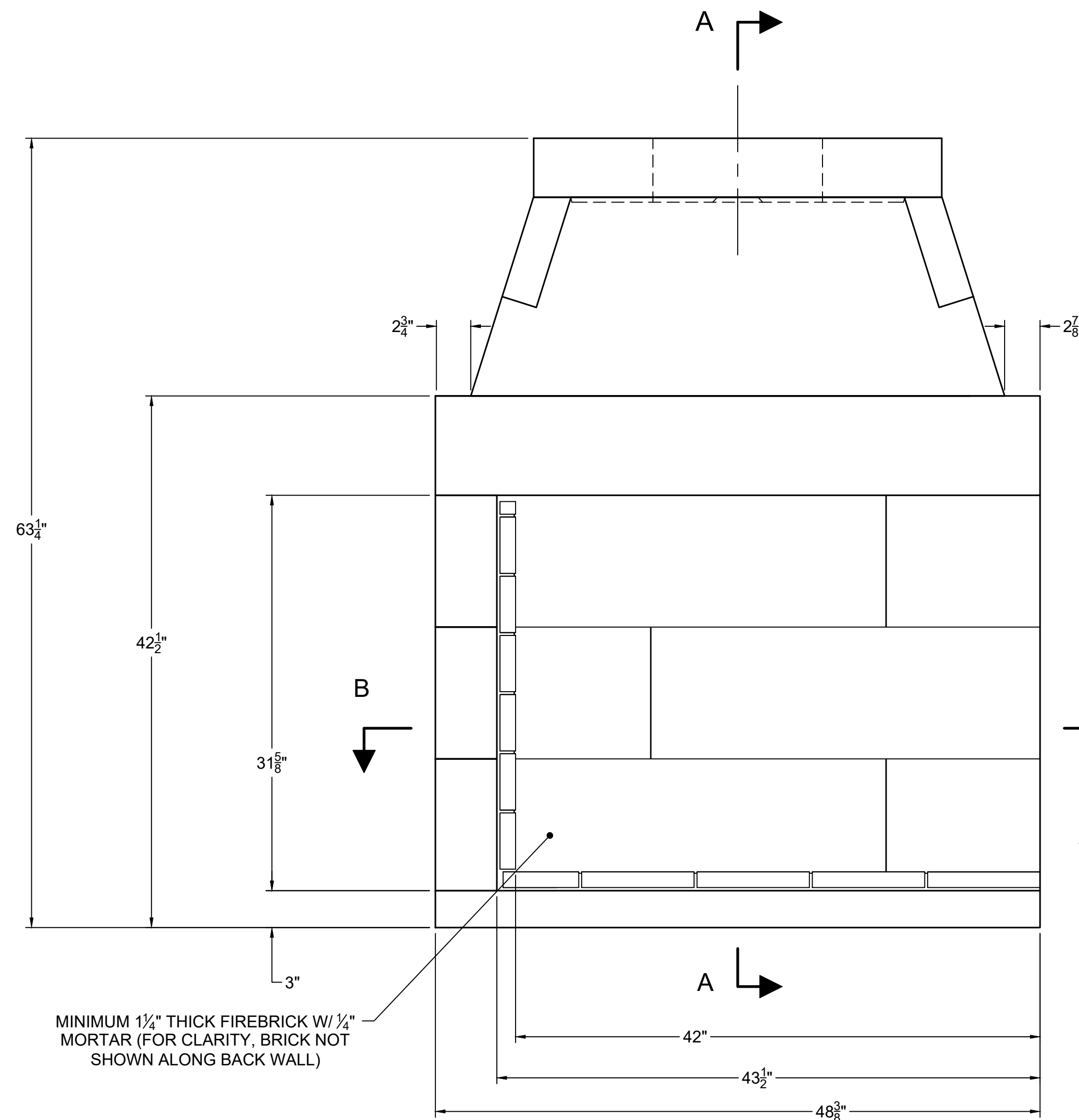
FRONT VIEW
